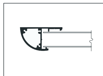
40mm Wall Channel with SignBar / Panel
