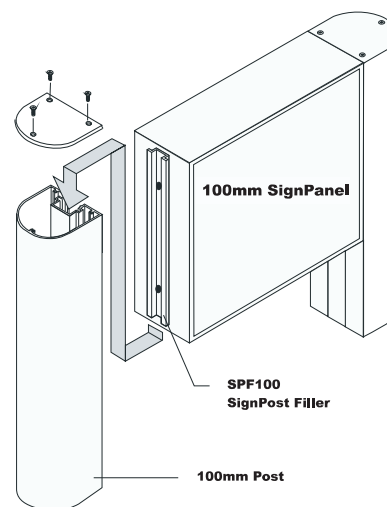
100mm SignPanel 100mm Post
