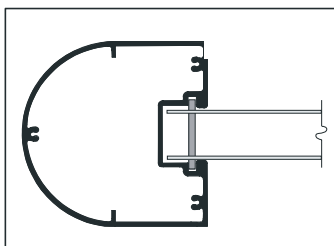
100mm Post with SignBar / Panel
